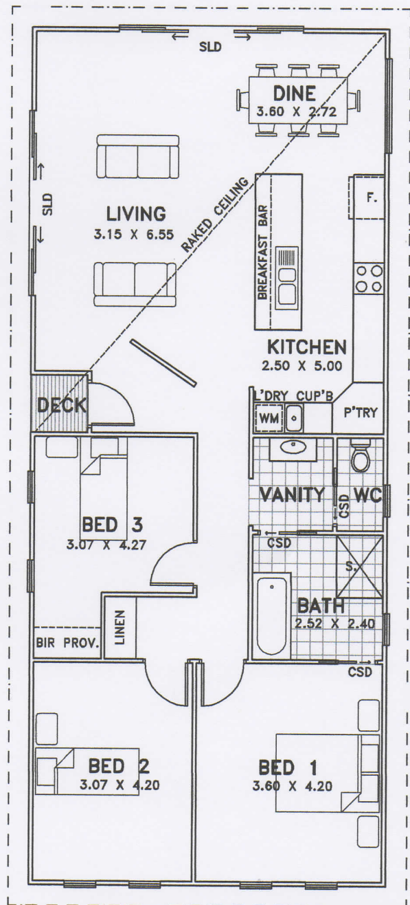
FLOOR PLAN
