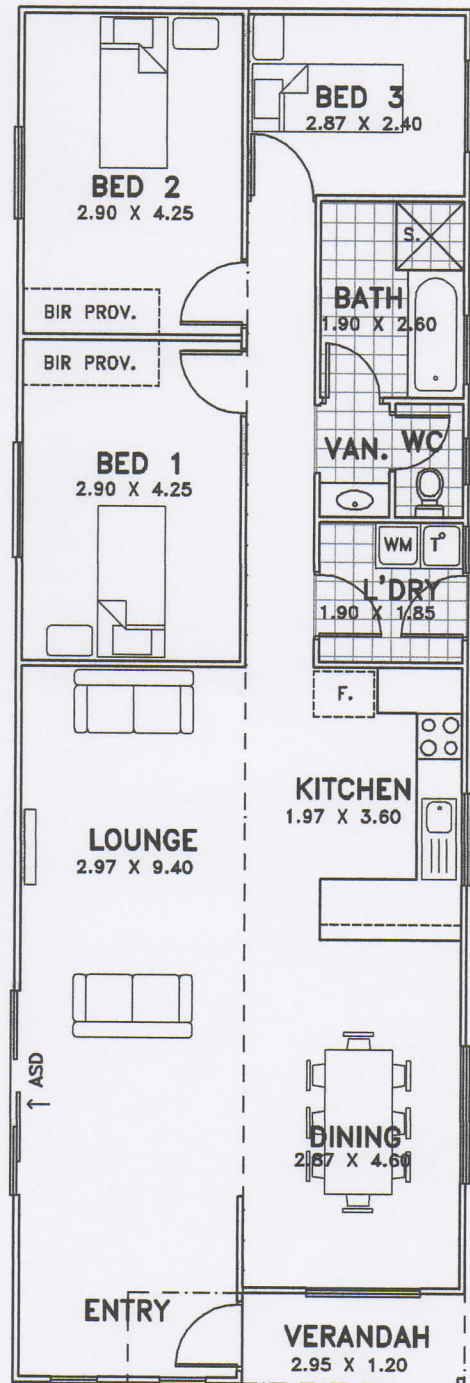
FLOOR PLAN
