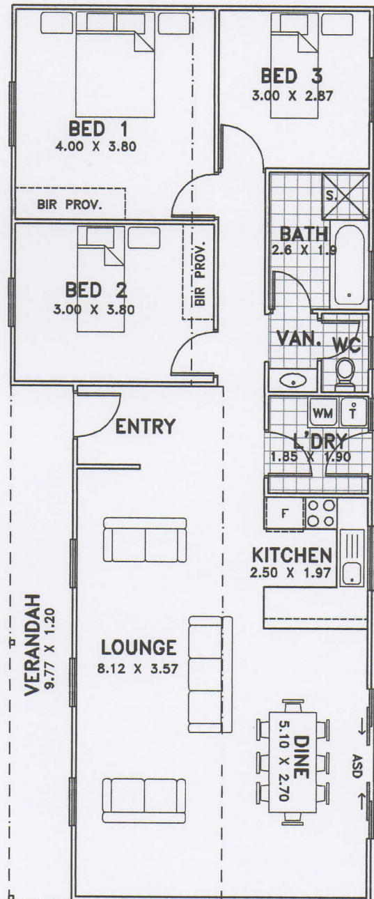
FLOOR PLAN
