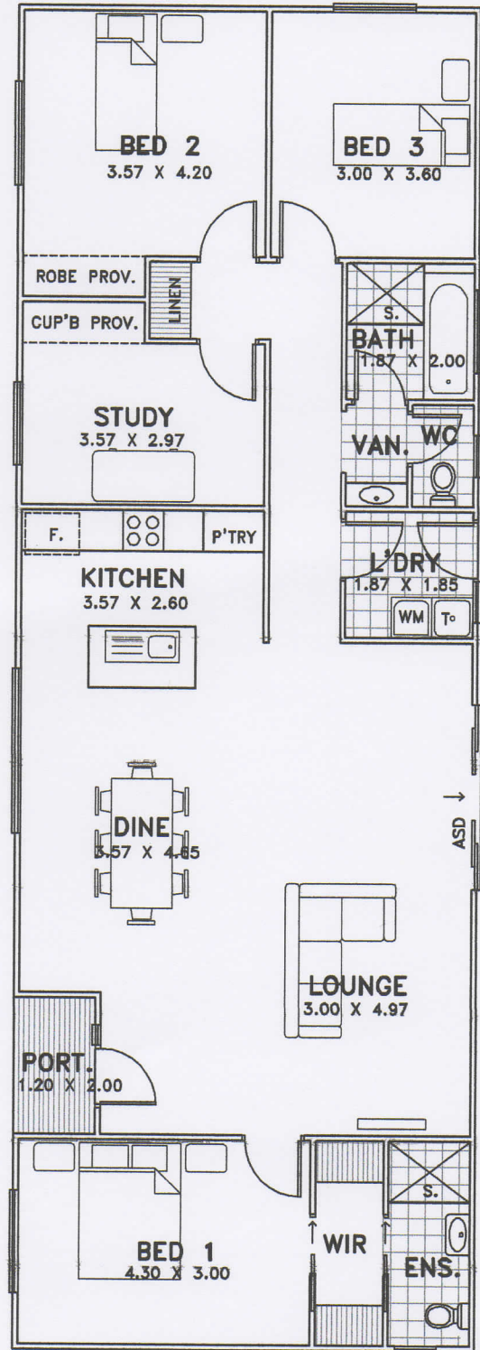
FLOOR PLAN
