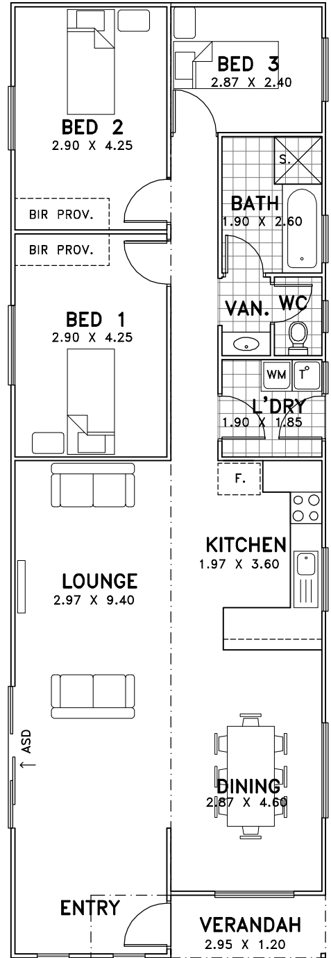
FLOOR PLAN
